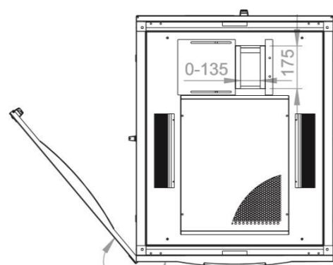
0°-230° Front door opening angle
