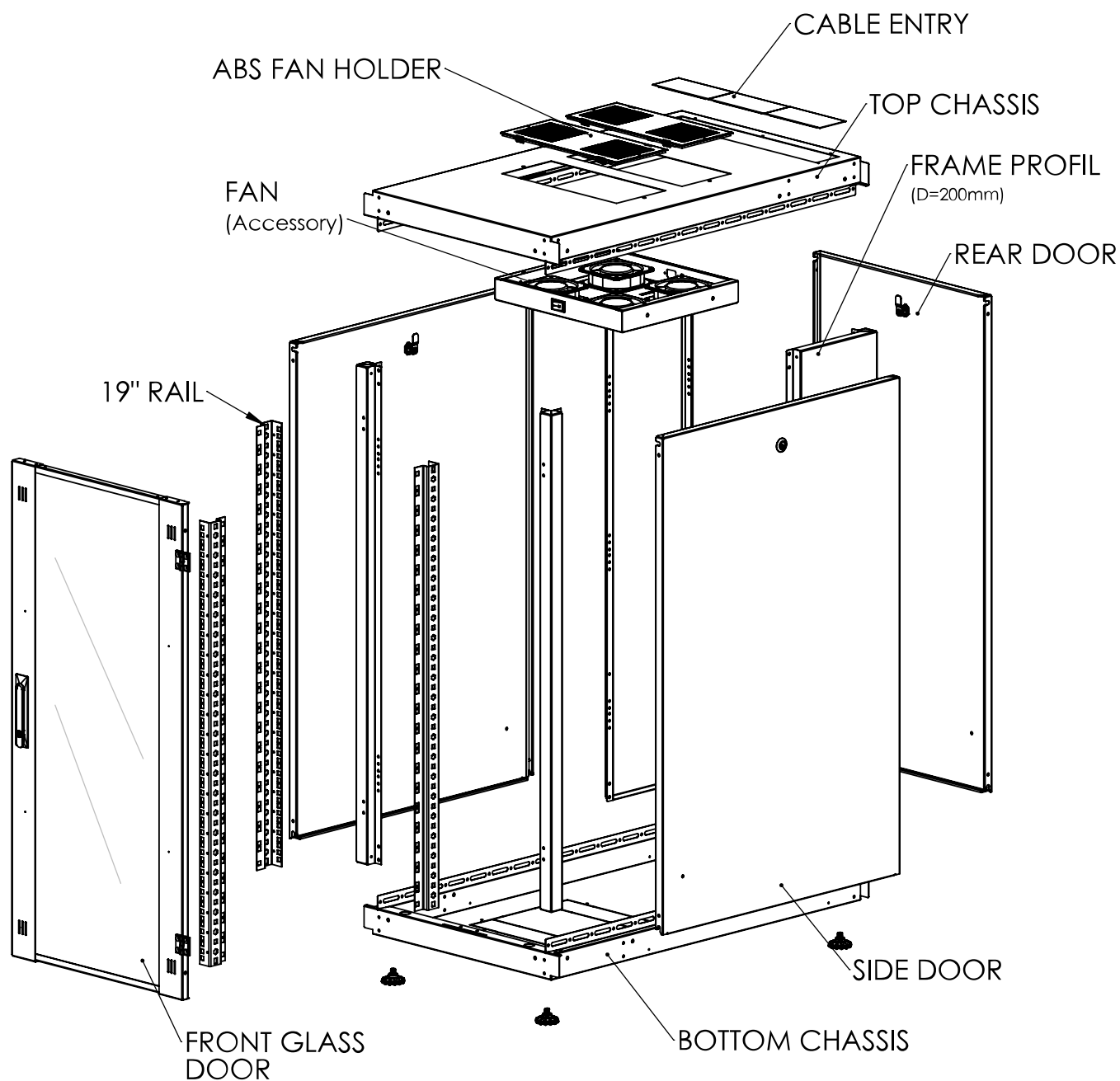
Exploded view
